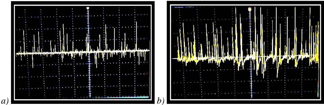
Fig. 6. Oscillograms of the motor magnetic field: a) in normal operation; b) in overload
