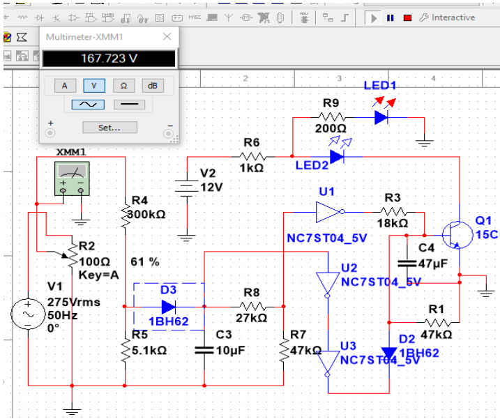
Fig. 9. Electrical circuit of the protection device at a voltage below the nominal value ( U_{in} < 168 \text{ V} )
