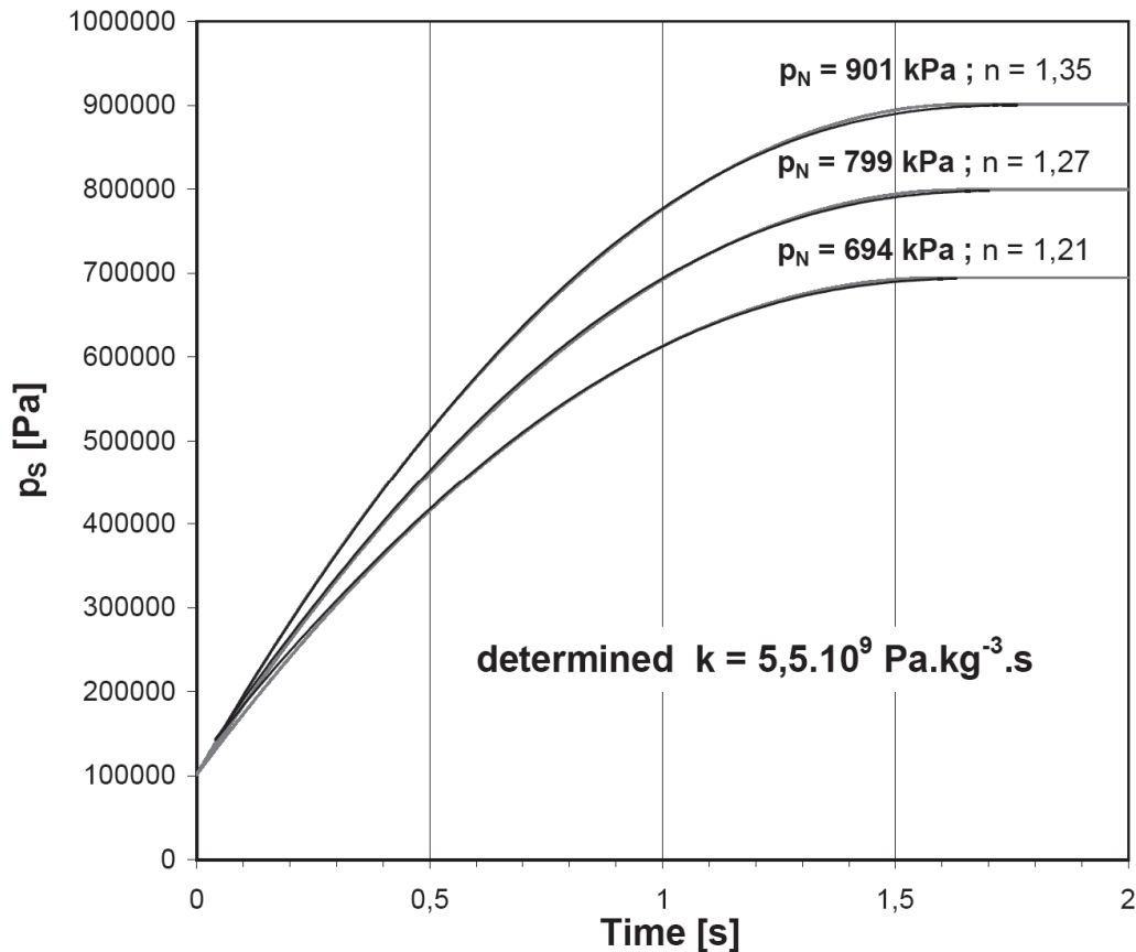
Fig. 4. Measured (black) and computed (grey) time dependences of absolute air pressure increase in compression space of the pneumatic coupling type 3-1/110-T-C
